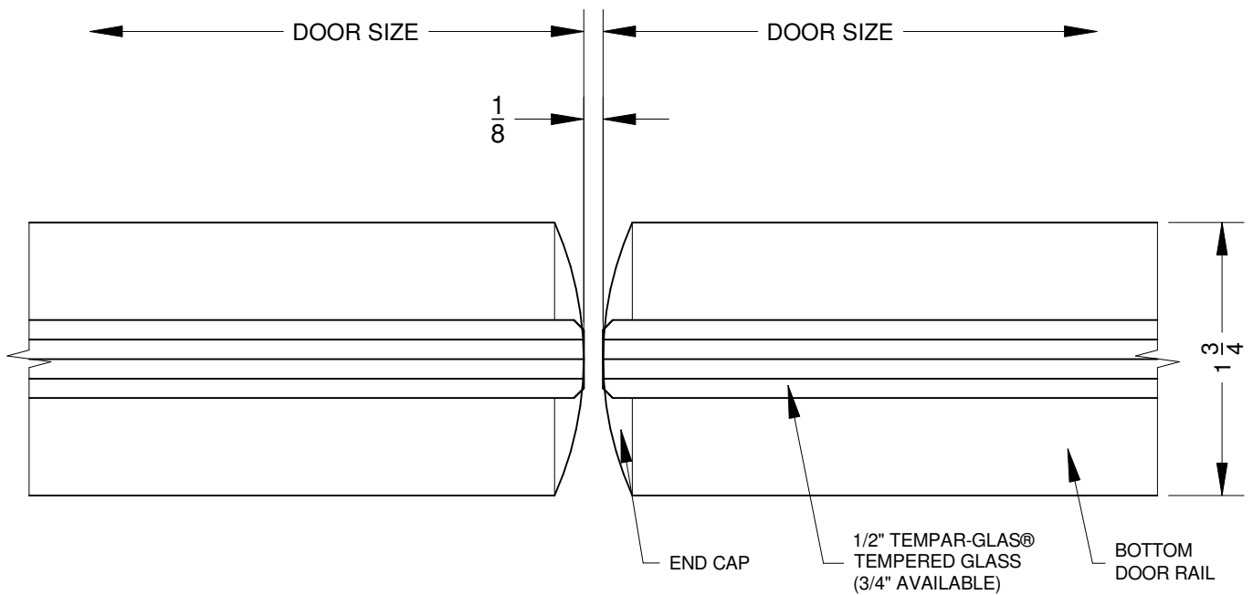
(B) - PLAN DETAIL AT MEETING JAMBS
