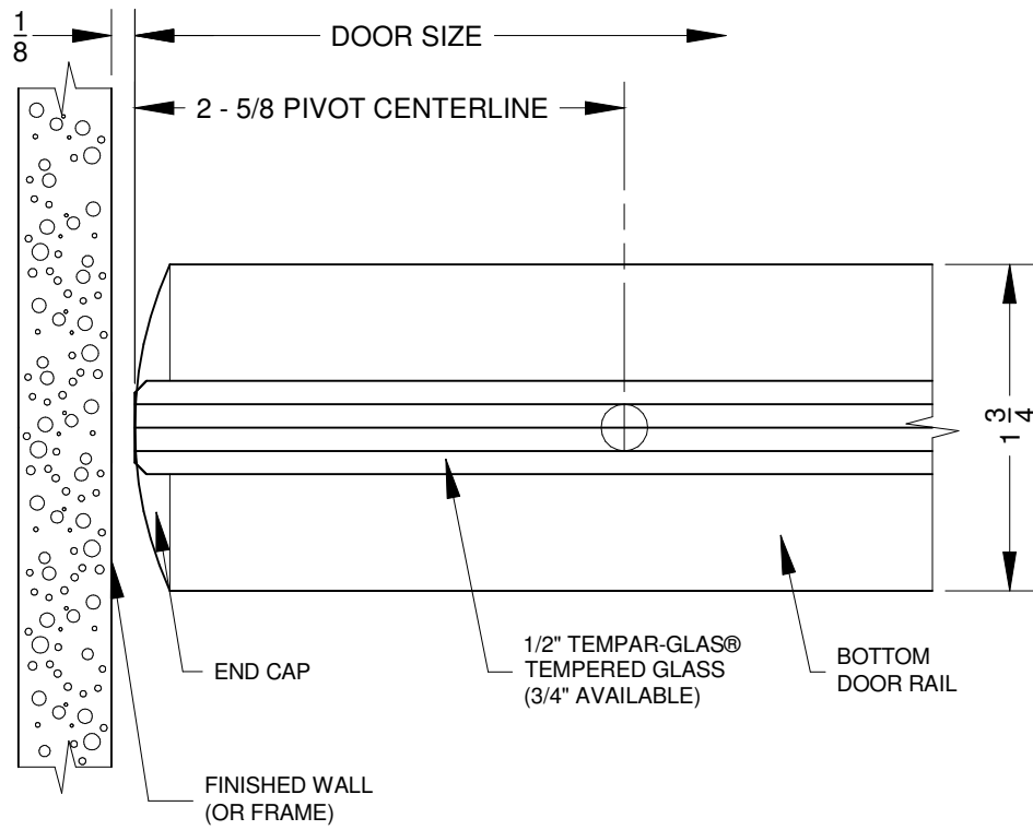
(A) - PLAN DETAIL AT WALL
